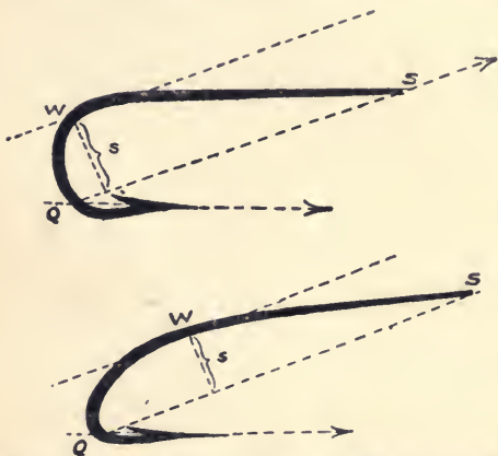
FIG. 7. Q S—Final line of pull. W—Weakest point so far as position only is concerned. s—Line of strength, with the length of which the likelihood of the hook to break at W increases.
